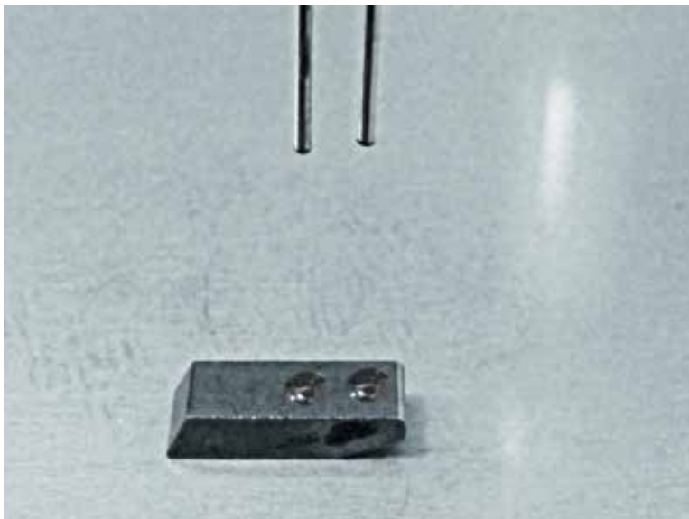
Tungsten carbide saw tooth: Flux paste F 300 DS 12 applied to a tungsten carbide surface
