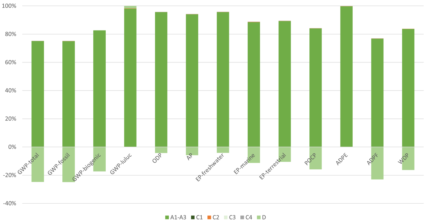
Hot-spot analysis of voestalpine roll-bonded clad plates (copper)
