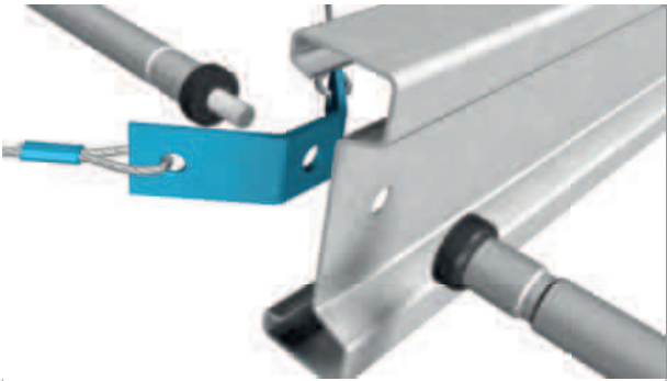
Montagedetail dakgording + Sadef-Lock® + dubbele bretel
