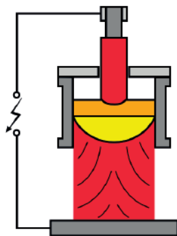
ESR: Electroslag Remelting Process
