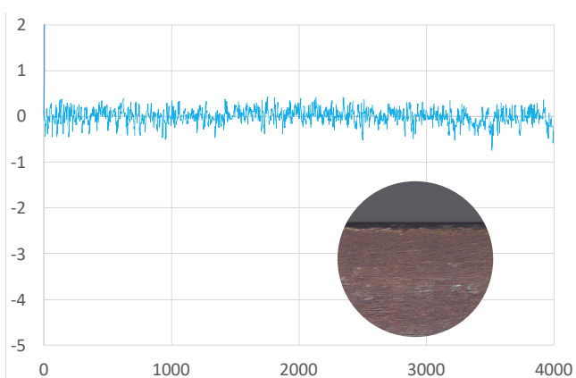
Same surface profile after polishing with #600 grit, R_a = 0,1 \mu\text{m} , R_z = 1,0 \mu\text{m}
