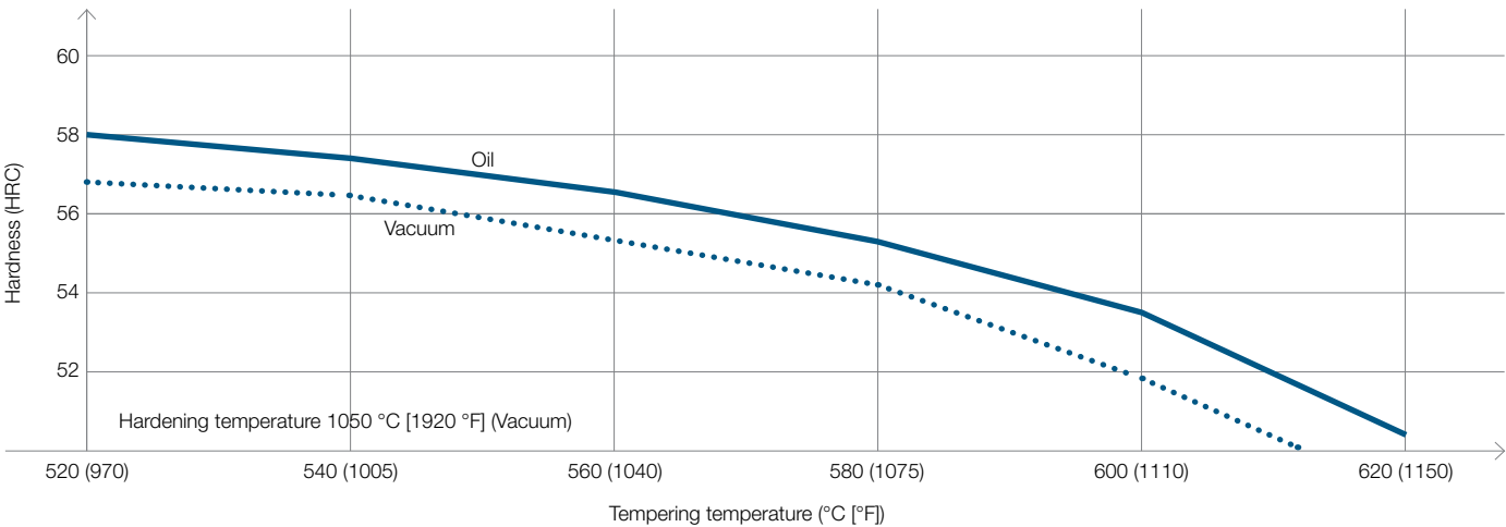
Tempering chart
