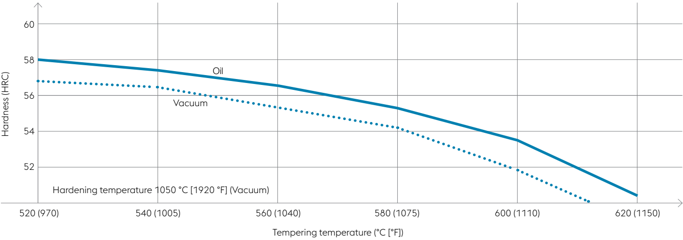
Tempering chart
