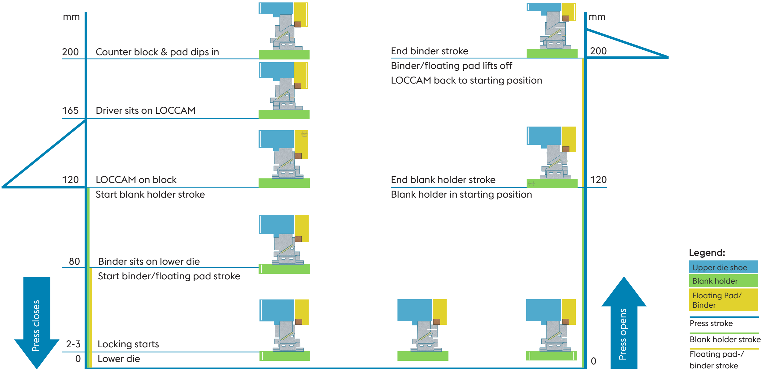
Blank holder with LOCCAM locked against binder/floating pad
