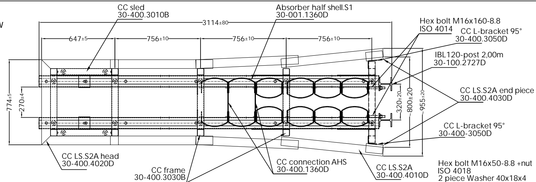
Side View
