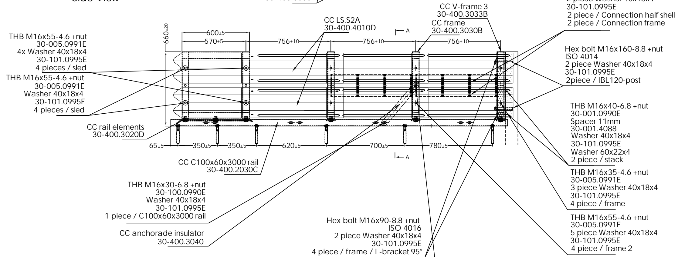
Section: A-A
